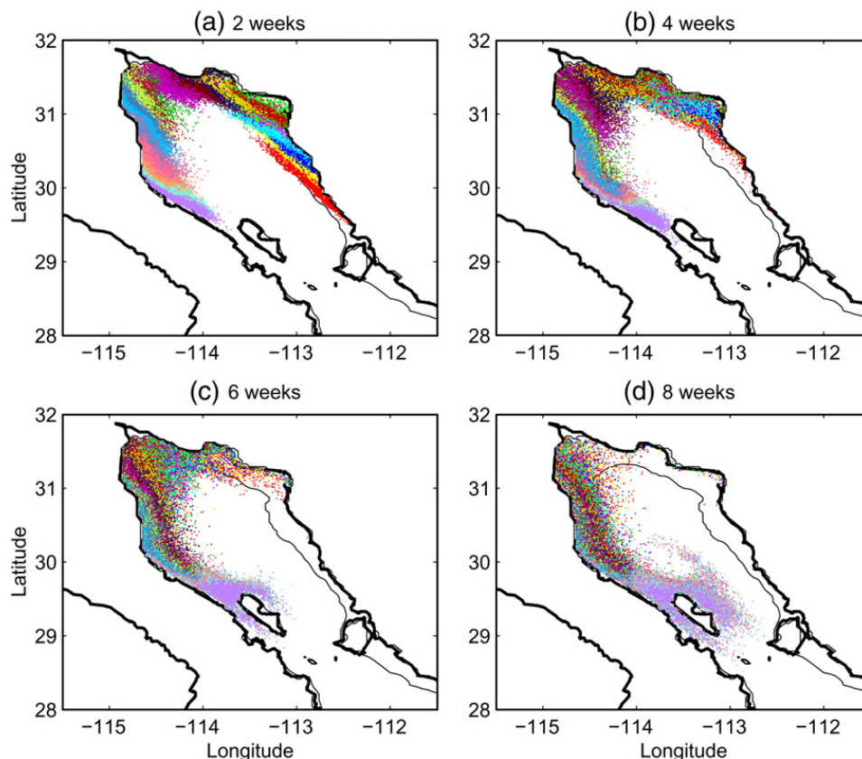
Fig. 4. Final position of the particles after (a) 2, (b) 4, (c) 6, and (d) 8 weeks. Their initial positions (21 positions areas) are shown in Fig. 1b. The 60 m isobath is shown.
