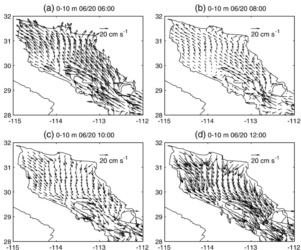
Fig. 3. Instantaneous currents for the first model layer (0–10 m) for June 20. Flood corresponds to hour (a) 6:00 and (b) 08:00 and ebb is occurring during hours (c) 10:00 and (d) 12:00. Only one in every three arrows is plotted for clarity.
