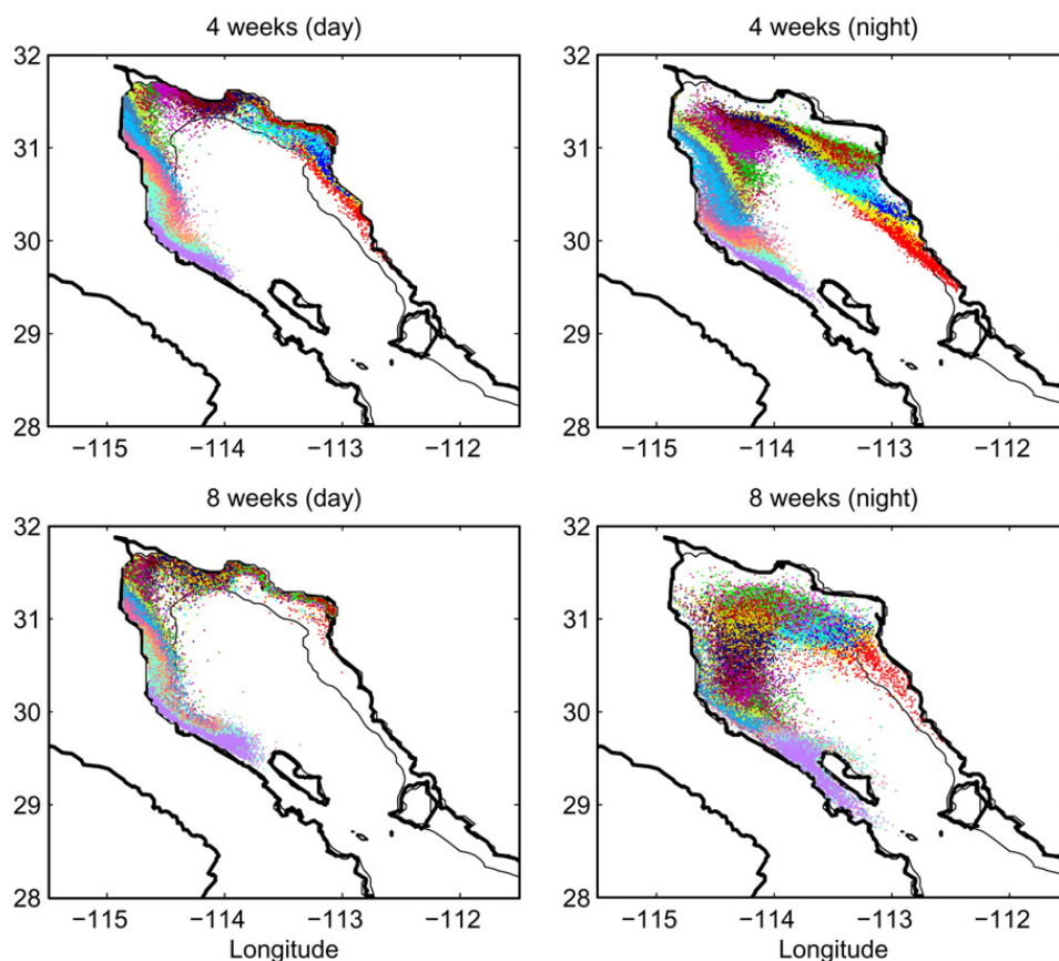
Fig. 7. Final position of the particles after 4 and 8 weeks. The left and right frames correspond to particles transported during day and during the night only, respectively. The 60 m isobath is shown.
