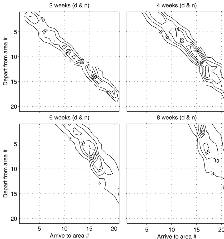
Fig. 5. Connectivity maps in (in percentage) after 2, 4, 6, and 8 weeks periods. The total number of particles seeded in each area is 2000 (a total of 21 \times 2000 ). The axes represent the area numbers given in Fig. 1: the vertical axes represent release areas, and the horizontal axes represent particle arrival areas.
